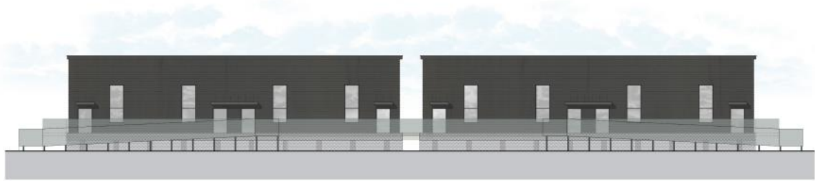
PROPOSED BACK ELEVATION UNITS 5&8 - 1/200 @ A1
